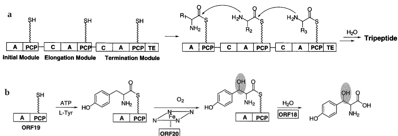
FIGURE 5: The role of paired A-PCP didomains: (a) Domain order and function in chain initiation, chain elongation, and chain termination modules of NRPS assembly lines. Amino acids are selected and activated by A domains and installed on the terminal thiol of phosphopantetheinyl arms on holo-PCP domains. C domains catalyze peptide bond condensation, and TE domains release the full-length peptidyl chains from the most downstream carrier protein site. (b) Proposed formation of (2S,3R)-3-OH-Tyr by the tandem action of ORF19 (A-PCP), ORF20 (heme hydroxylase), and ORF18 (TE) in glycopeptide antibiotic biosynthesis.
