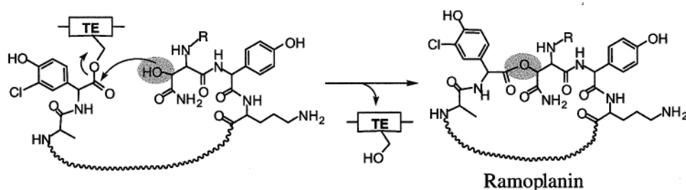
FIGURE 3: Reactions of the \beta -OH groups in peptide antibiotic maturation: (a) glycosylation of \beta -OH-Tyr 6 with TDP-L-epivancosamine by a dedicated glycosyl transferase in chloroeremomycin biosynthesis; (b) oxidation of the \beta -OH-tyrosyl-S-enzyme during novobiocin assembly; (c) retro-aldol cleavage of \beta -OH-His during imidazolone aldehyde formation in nikkomycin X biosynthesis; (d) macrolactone ring formation by the thioesterase domain of ramoplanin synthetase.
