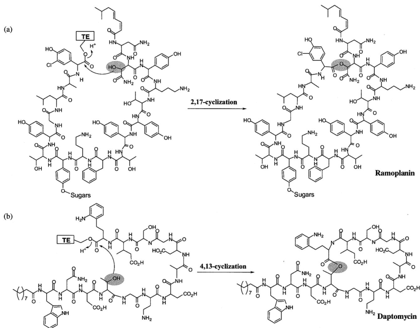
FIGURE 4: Macrocyclization of peptidyl-O-TE acyl-enzyme intermediates during construction of the macrolactone scaffold of peptidolactone antibiotics: (a) attack of the \beta -OH side chain of \beta -OH-Asn 2 on the carbonyl of 3-Cl-4-OH-PheGly 17 in the peptidyl-O-TE domain acyl-enzyme of ramoplanin synthetase; (b) attack of the \beta -OH side chain of Thr 4 on the carbonyl of Kyn 13 in the peptidyl-O-TE domain acyl-enzyme of daptomycin synthetase.
